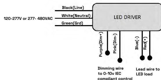
General Wiring Diagram
