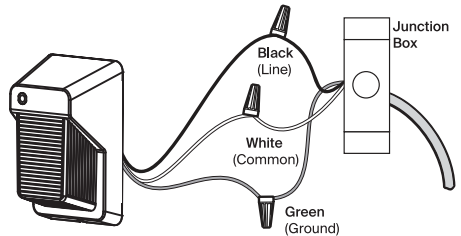
Wiring Diagram
