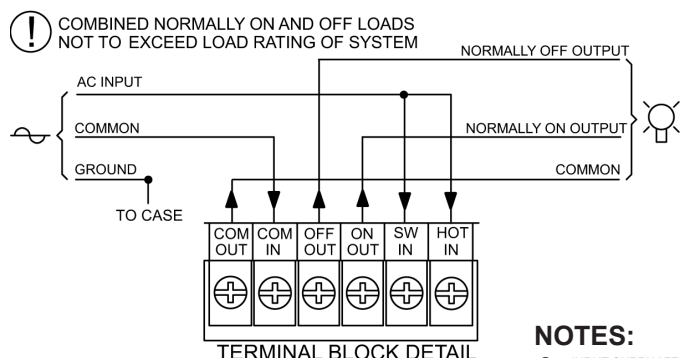
Diagram 3. NORMALLY ON & OFF LOADS
